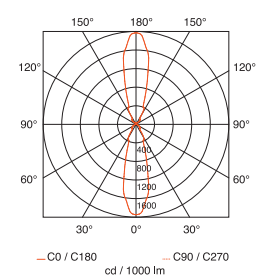
Par-30 75W
