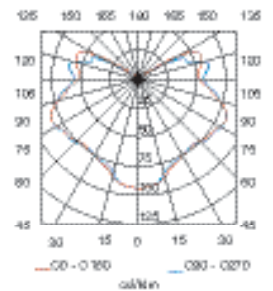
E-27 100W
