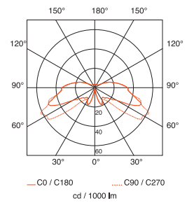
GU-10 50W
