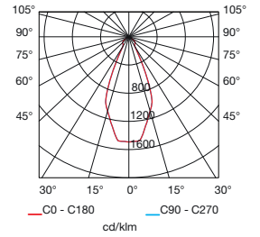
GU-10 50W
