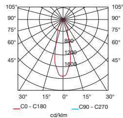
Par-30 75W
